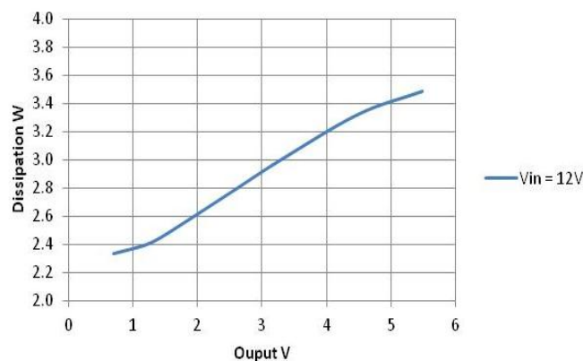
Figure 5 Dissipation vs Voltage. I_{out} = 7 A, F_{sw} = 500 kHz
