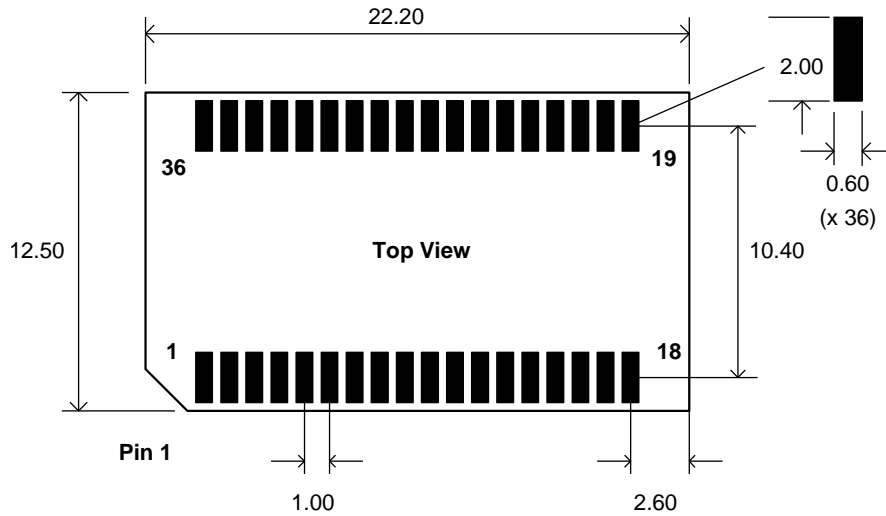
Figure 54. Recommended PCB Pad Sizes
