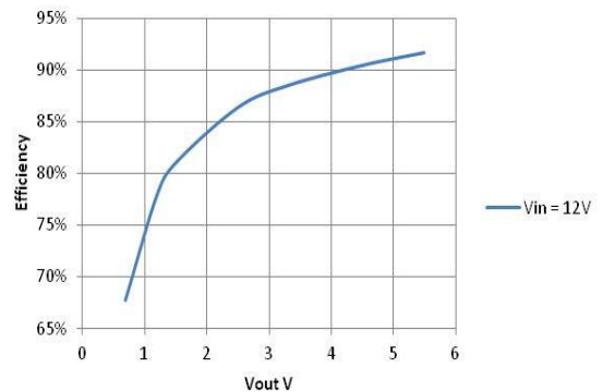
Figure 4 Efficiency vs. Output Voltage, I_{out} = 7 A, F_{sw} = 500 kHz
