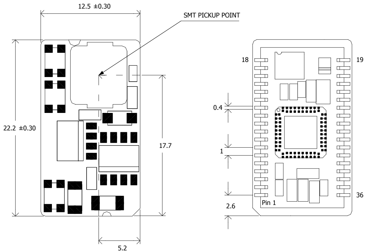
Figure 51. Top (Left) and Bottom Views
