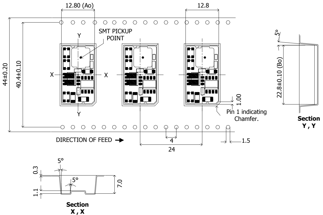
Figure 53. Tape and Reel
