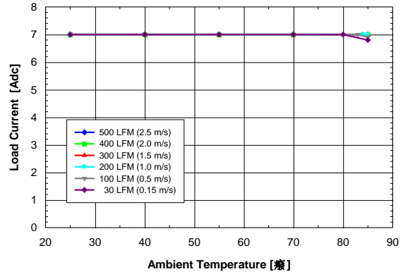
Figure 2 Available output current vs. ambient air temperature and airflow rates for converter DP7007G mounted horizontally with air flowing from input to output, MOSFET temperature \leq 120 °C, V_{in} = 12 V, V_{out} = 5 V, and F_{sw} = 1 MHz
