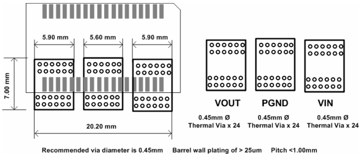
Figure 55. Recommended PCB Layout for Multilayer PCBs
