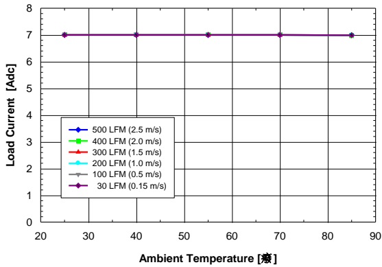
Figure 1 Available output current vs. ambient air temperature and airflow rates for converter DP7007G mounted horizontally with air flowing from input to output, MOSFET temperature \leq 120 °C, V_{in} = 12 V, V_{out} = 5 V, and F_{sw} = 500 kHz
