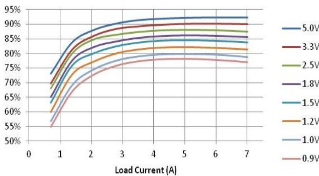
Figure 3 Efficiency vs. Load. V_{in} = 12 V, F_{sw} = 500 kHz
