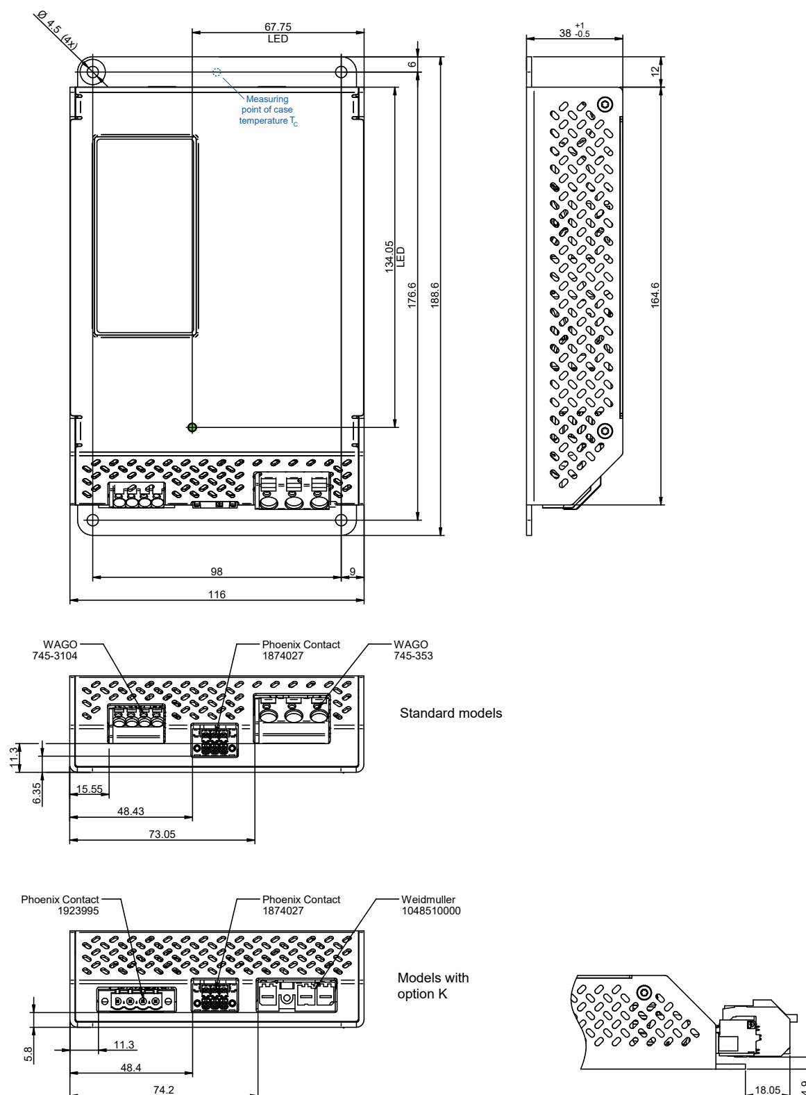
Fig. 8 Case of RCM200/300 (RCM02) weight approx. 820 g, Aluminum, EP-powder coated
