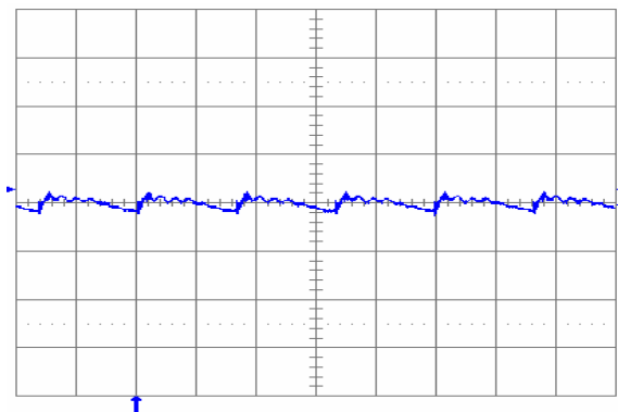
Fig. 1.0V.6: Output voltage ripple (20 mV/div.) at full rated load current into a resistive load with external capacitance 100 \mu F ceramic + 1 \mu F ceramic, and V_{in} = 12 V for V_{out} = 1.0 V. Time scale: 2 \mu s/div.
