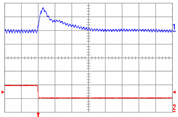
Fig. 1.8V.8: Output voltage response for V_{out} = 1.8 V to negative load current step change from 10 A to 5 A with slew rate of -5 \text{ A}/\mu\text{s} at V_{in} = 5 V. Top trace: output voltage (100 mV/div.); Bottom trace: load current (5 A/div.). C_o = 100 \mu\text{F} ceramic + 1 \mu\text{F} ceramic. Time scale: 20 \mu\text{s}/\text{div} .
