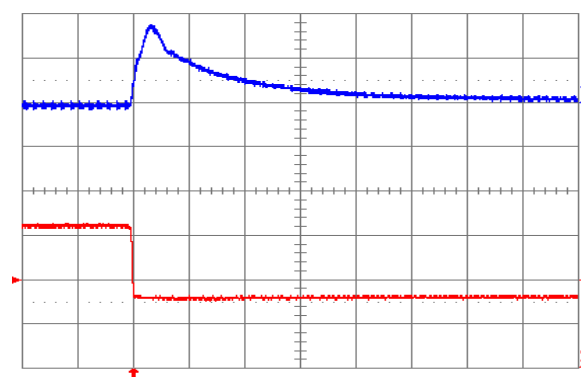
Fig. 0.7525V.8: Output voltage response for V_{out} = 0.7525 V to negative load current step change from 16 A to 8 A with slew rate of -5\text{ A}/\mu\text{s} at V_{in} = 5 V. Top trace: output voltage (100 mV/div.); Bottom trace: load current (5 A/div.). C_o = 100\text{ }\mu\text{F} ceramic. Time scale: 20 \mu\text{s} /div.
