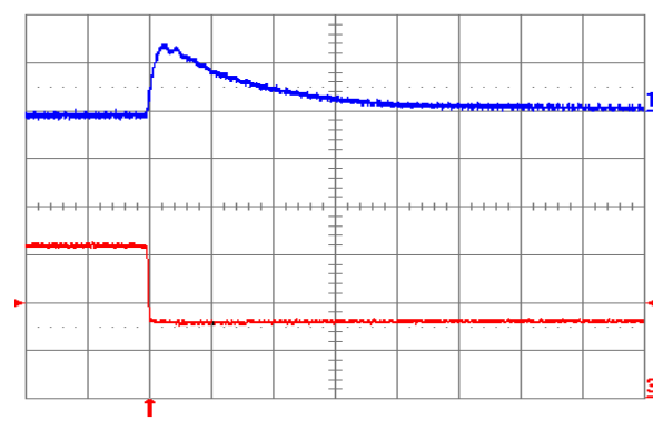
Fig. 1.8V.8: Output voltage response for V_{out} = 1.8 V to negative load current step change from 16 A to 8 A with slew rate of -5\text{ A}/\mu\text{s} at V_{in} = 5 V. Top trace: output voltage (100 mV/div.); Bottom trace: load current (5 A/div.). C_o = 100\mu\text{F} ceramic. Time scale: 20 \mu\text{s} /div.
