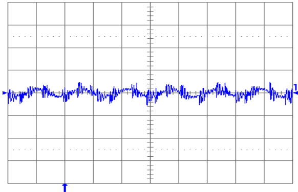
Fig. 2.0V.6: Output voltage ripple (20 mV/div.) at full rated load current into a resistive load with external capacitance 100 \mu F ceramic + 1 \mu F ceramic and V_{in} = 5 V for V_{out} = 2.0 V. Time scale: 2 \mu s/div.
