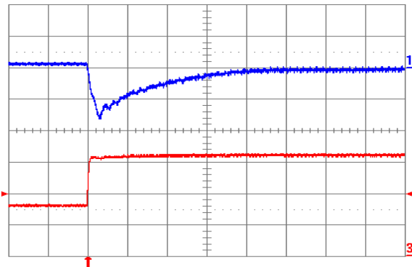
Fig. 2.5V.7: Output voltage response for V_{out} = 2.5 V to positive load current step change from 8 A to 16 A with slew rate of 5 A/ \mu s at V_{in} = 5 V. Top trace: output voltage (100 mV/div.); Bottom trace: load current (5 A/div.). C_o = 100 \mu F ceramic. Time scale: 20 \mu s/div.
