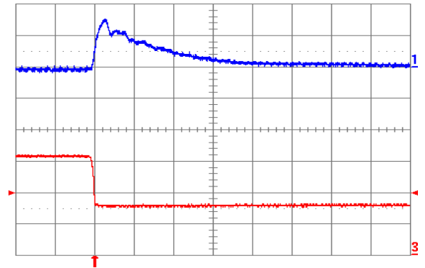
Fig. 3.3V.8: Output voltage response for V_{out} = 3.3 V to negative load current step change from 16 A to 8 A with slew rate of -5 A/ \mu s at V_{in} = 5 V. Top trace: output voltage (100 mV/div.); Bottom trace: load current (5 A/div.). C_o = 100 \mu F ceramic. Time scale: 20 \mu s/div.
