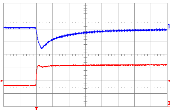
Fig. 0.7525V.7: Output voltage response for V_{out} = 0.7525 V to positive load current step change from 8 A to 16 A with slew rate of 5\text{ A}/\mu\text{s} at V_{in} = 5 V. Top trace: output voltage (100 mV/div.); Bottom trace: load current (5 A/div.). C_o = 100\text{ }\mu\text{F} ceramic. Time scale: 20 \mu\text{s} /div.
