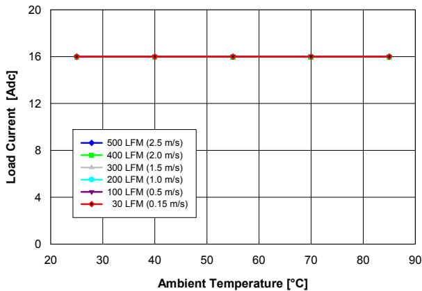
Fig. 0.7525V.1: Available load current vs. ambient temperature and airflow rates for Vout = 0.7525 V converter mounted vertically with Vin = 5 V, and maximum MOSFET temperature ≤ 120 °C.
