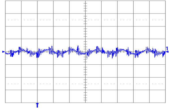
Fig. 1.8V.6: Output voltage ripple (20 mV/div.) at full rated load current into a resistive load with external capacitance 100\mu\text{F} ceramic + 1\mu\text{F} ceramic and V_{in} = 5 V for V_{out} = 1.8 V. Time scale: 2 \mu\text{s} /div.
