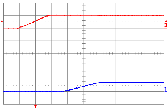
Fig. 0.7525V.5: Turn-on transient for V_{out} = 0.7525 V with application of V_{in} at full rated load current (resistive) and 100\text{ }\mu\text{F} external capacitance at V_{in} = 5 V. Top trace: V_{in} (5 V/div.); Bottom trace: output voltage (1 V/div.); Time scale: 2 ms/div.
