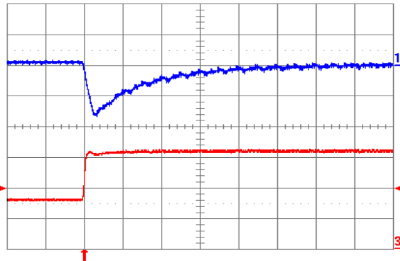
Fig. 1.2V.7: Output voltage response for V_{out} = 1.2 V to positive load current step change from 8 A to 16 A with slew rate of 5 A/ \mu s at V_{in} = 5 V. Top trace: output voltage (100 mV/div.); Bottom trace: load current (5 A/div.). C_o = 100 \mu F ceramic. Time scale: 20 \mu s/div.
