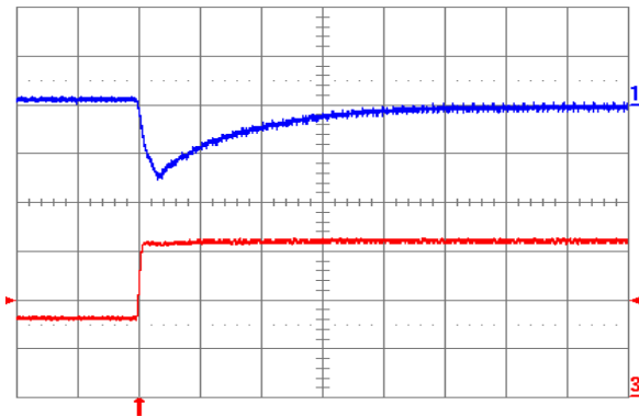
Fig. 1.8V.7: Output voltage response for V_{out} = 1.8 V to positive load current step change from 8 A to 16 A with slew rate of 5\text{ A}/\mu\text{s} at V_{in} = 5 V. Top trace: output voltage (100 mV/div.); Bottom trace: load current (5 A/div.). C_o = 100\mu\text{F} ceramic. Time scale: 20 \mu\text{s} /div.
