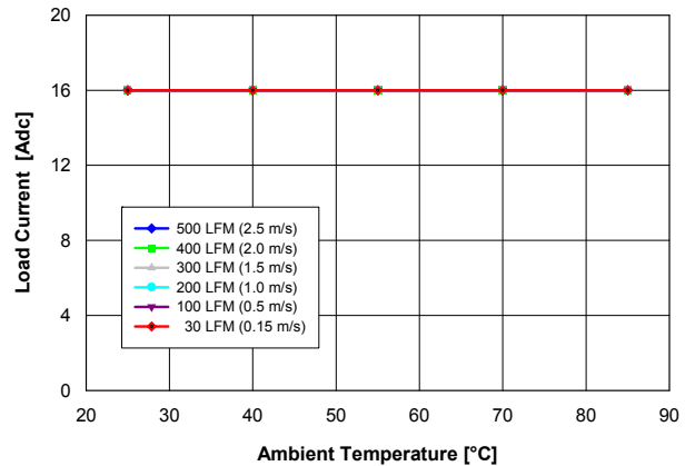
Fig. 0.7525V.2: Available load current vs. ambient temperature and airflow rates for Vout = 0.7525 V converter mounted horizontally with Vin = 5 V, and maximum MOSFET temperature ≤ 120 °C.
