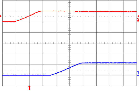
Fig. 1.2V.5: Turn-on transient for V_{out} = 1.2 V with application of V_{in} at full rated load current (resistive) and 100 \mu F external capacitance at V_{in} = 5 V. Top trace: V_{in} (5 V/div.); Bottom trace: output voltage (1 V/div.); Time scale: 2 ms/div.
