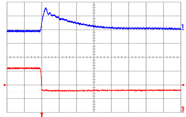
Fig. 2.5V.8: Output voltage response for V_{out} = 2.5 V to negative load current step change from 16 A to 8 A with slew rate of -5 A/ \mu s at V_{in} = 5 V. Top trace: output voltage (100 mV/div.); Bottom trace: load current (5 A/div.). C_o = 100 \mu F ceramic. Time scale: 20 \mu s/div.
