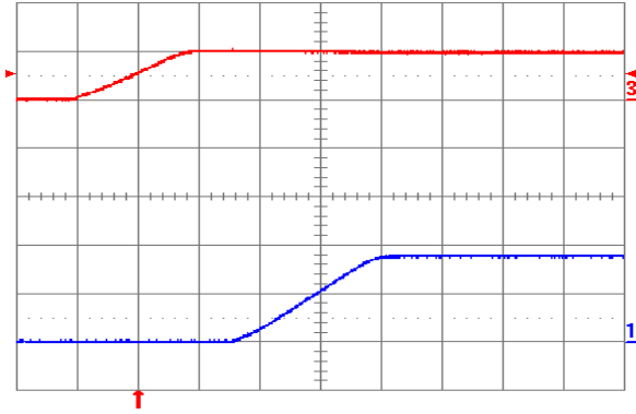
Fig. 1.8V.5: Turn-on transient for V_{out} = 1.8 V with application of V_{in} at full rated load current (resistive) and 100\mu\text{F} external capacitance at V_{in} = 5 V. Top trace: V_{in} (5 V/div.); Bottom trace: output voltage (1V/div.); Time scale: 2 ms/div.
