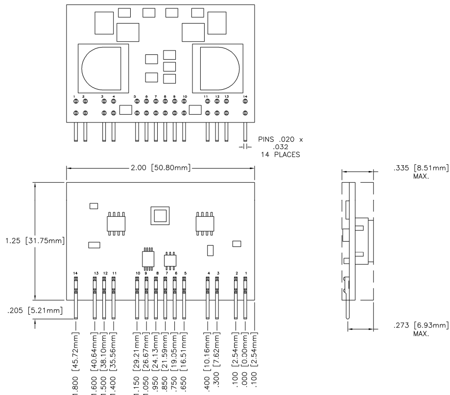
Through-hole – SIP
