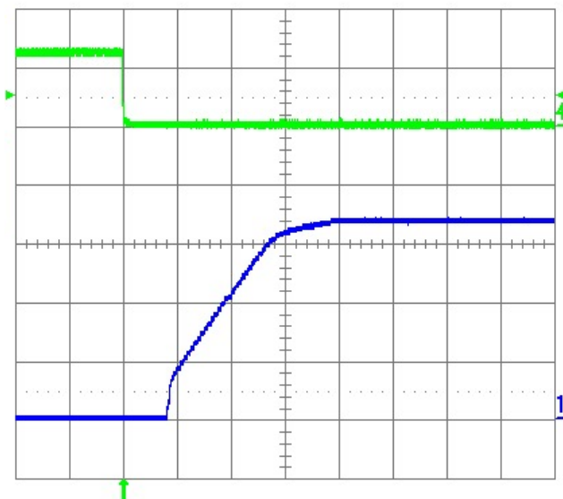
Fig. 17: Turn-on transient for V_{out} = 3.3\text{ V} with the application of SEQ/ENA signal at full rated load current (resistive) and 1\text{ }\mu\text{F} external capacitance at V_{in} = 12\text{ V} . Top Trace: SEQ/ENA Signal (5 V/div.); Bottom Trace: Output Voltage (1 V/div.); Time Scale: 1 ms/div.
