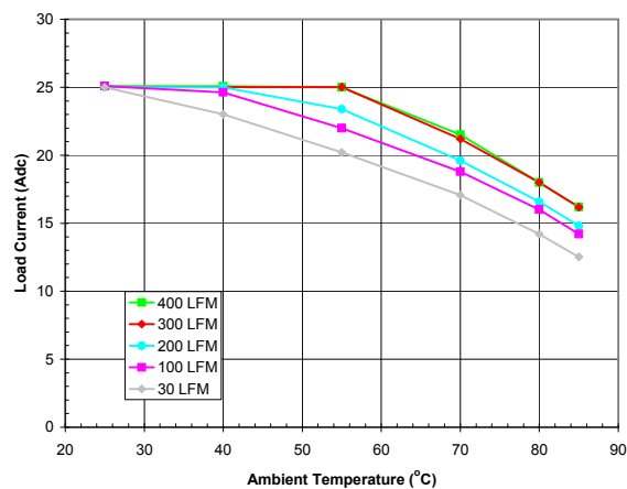
Fig. 16: Available load current vs. ambient temperature and airflow rates for V_{out} = 1.2 V with V_{in} = 12 V, and maximum MOSFET temperature \leq 110 °C. Horizontal Orientation (Airflow from Vin pin to GND pin.)
