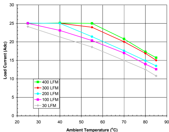
Fig. 13: Available load current vs. ambient temperature and airflow rates for V_{out} = 5.0 V with V_{in} = 12 V, and maximum MOSFET temperature \leq 110 °C. Horizontal Orientation (Airflow from Vin pin to GND pin.)
