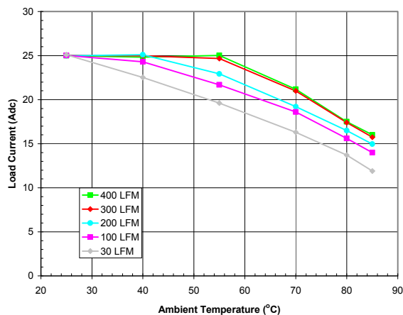
Fig. 15: Available load current vs. ambient temperature and airflow rates for V_{out} = 1.8 V with V_{in} = 12 V, and maximum MOSFET temperature \leq 110 °C. Horizontal Orientation (Airflow from Vin pin to GND pin.)
