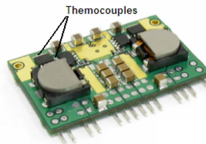
Fig. D: Location of the thermocouples for thermal testing.
