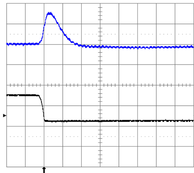
Fig. 24: Output voltage response for V_{out} = 3.3 V to negative load current step change from 25 A to 12.5 A with slew rate of -5 A/ \mu s at V_{in} = 12 V. Top Trace: Output Voltage (100 mV/div.); Bottom Trace: Load Current (10 A/div.) C_o = 1 \mu F ceramic. Time Scale: 10 \mu s/div.
