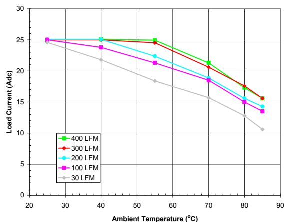
Fig. 14: Available load current vs. ambient temperature and airflow rates for V_{out} = 3.3 V with V_{in} = 12 V, and maximum MOSFET temperature \leq 110 °C. Horizontal Orientation (Airflow from Vin pin to GND pin.)
