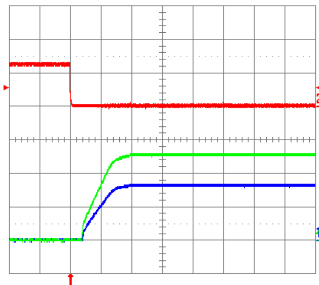
Fig. 18: Turn-on transient for V_{out} = 3.3\text{ V} and 5.0\text{ V} with the application of SEQ/ENA signal at full rated load current (resistive) and 1\text{ }\mu\text{F} external capacitance at V_{in} = 12\text{ V} . SEQ/ENA pins are tied together. Top Trace: SEQ/ENA Signal (5 V/div.); Middle Trace: Output Voltage of 5V POL (2V/div.); Bottom Trace: Output Voltage of 3.3V POL (2 V/div.); Time Scale: 2 ms/div.
