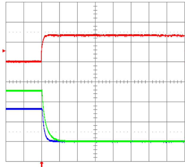
Fig. 20: Turn-off transient for V_{out} = 3.3\text{ V} and 5.0\text{ V} with the removal of SEQ/ENA signal at full rated load current (resistive) and 1\text{ }\mu\text{F} external capacitance at V_{in} = 12\text{ V} . SEQ/ENA pins are tied together. Top Trace: SEQ/ENA Signal (5 V/div.); Middle Trace: Output Voltage of 5V POL (2V/div.); Bottom Trace: Output Voltage of 3.3V POL (2 V/div.); Time Scale: 2 ms/div.
