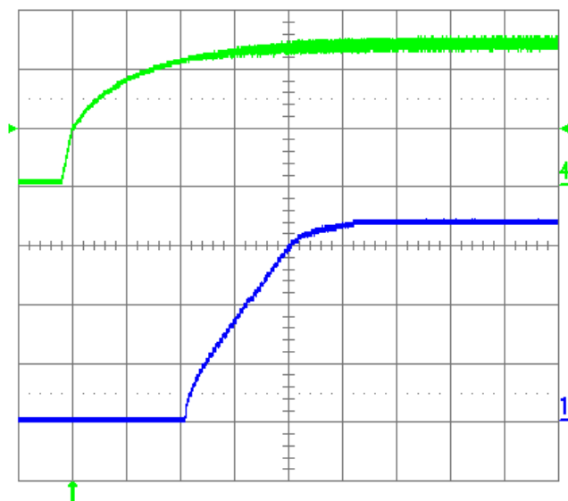
Fig. 19: Turn-on transient for V_{out} = 3.3\text{ V} with the application of the input voltage at full rated load current (resistive) and 1\text{ }\mu\text{F} external capacitance at V_{in} = 12\text{ V} . Top Trace: Input Voltage Signal (5 V/div.); Bottom Trace: Output Voltage (1 V/div.); Time Scale: 1 ms/div.
