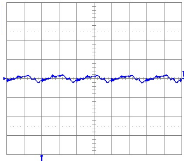
Fig. 21: Output voltage ripple (20 mV/div.) at full rated load current into a resistive load with external capacitance 1 \mu F ceramic and V_{in} = 12 V for V_{out} = 3.3 V. Time Scale: 1 \mu s/div.
