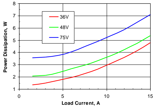
Figure 4. Power dissipation vs. load current and input voltage for SSQE48T15033 converter mounted vertically with air flowing from pin 1 to pin 3 at a rate of 300 LFM (1.5 m/s) and T_a = 25\text{ °C}
