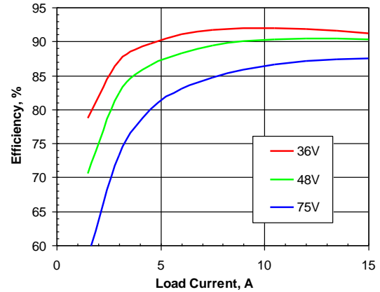
Figure 2. Efficiency vs. load current and input voltage for SSQE48T15033 converter mounted vertically with air flowing from pin 1 to pin 3 at a rate of 300 LFM (1.5 m/s) and T_a = 25\text{ °C} .
