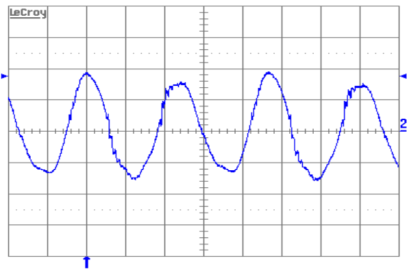
Figure 10. Output voltage ripple (20 mV/div.) at full rated load current into a resistive load with C_o = 10\mu\text{F} tantalum + 1\mu\text{F} ceramic and V_{in} = 48\text{ V} . Time scale: 1 \mu\text{s}/\text{div} .
