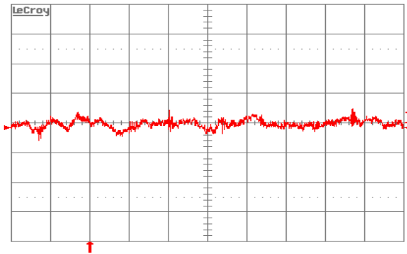
Figure 12. Input reflected-ripple current, i_s (10mA/div.), measured through 10\mu\text{H} at the source at full rated load current and V_{in} = 48\text{V} . Refer to Figure 11 for test setup. Time scale: 1\mu\text{s}/\text{div} .
