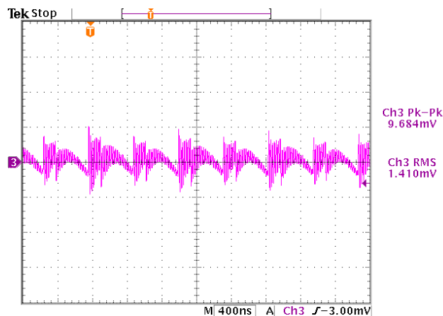
Figure 42. Output Voltage Noise, Full Load, 180° Interleave
