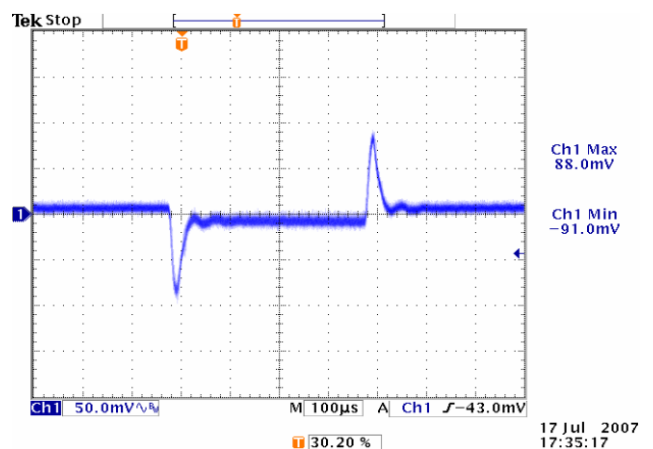
Figure 13. Vin=12V, Vout=1.8V
