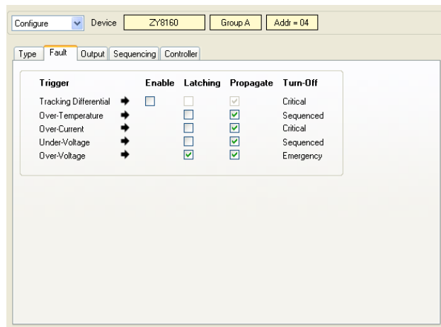
Figure 30. Fault management window
