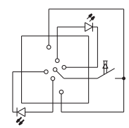
Keyswitch, fully illuminated
