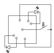
Keyswitch, spot-illuminated
