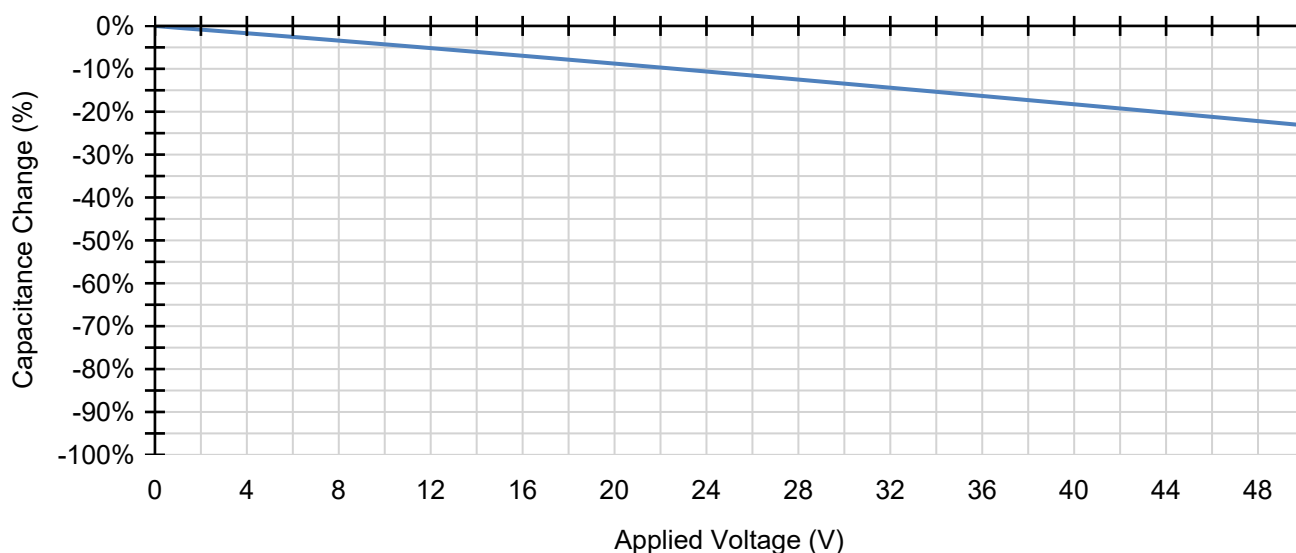
VCC Characterization
