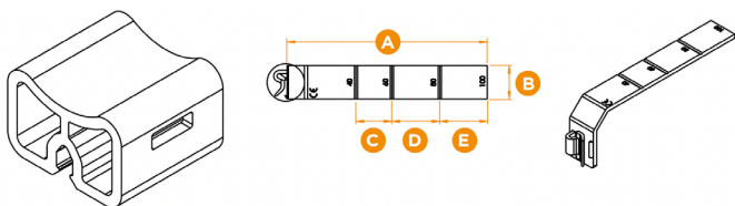
Cable Holder
