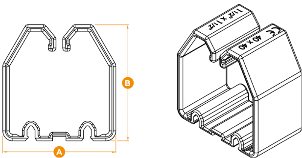
Wire retainer
