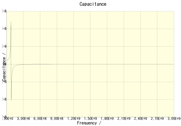
C2012C0G2A472J125AA
