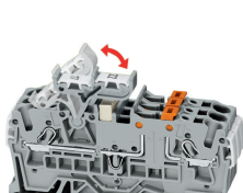
Pivoting double-deck marker carrier (2002-121) and 2-conductor disconnect/ test terminal block (2002-1671)
