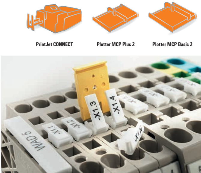
Foldable hinges for easy assembly of cross-connectors; shield lengths of up to 15 mm for long series of characters.
