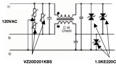
MOV In AC Line Protection
