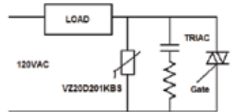
MOV in Triac Protection
