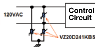
MOV In Control Circuit Protection
