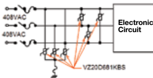
MOV for 3 Phase AC Line Protection
