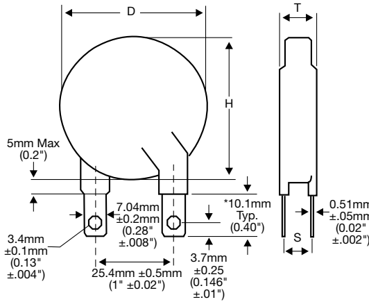
Uncoated Disk Part Number Suffix “KR”
