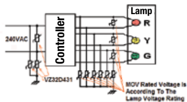
MOV In Traffic Light Protection
