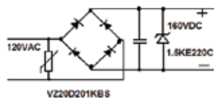
MOV in Bridge Rectifier Protection
