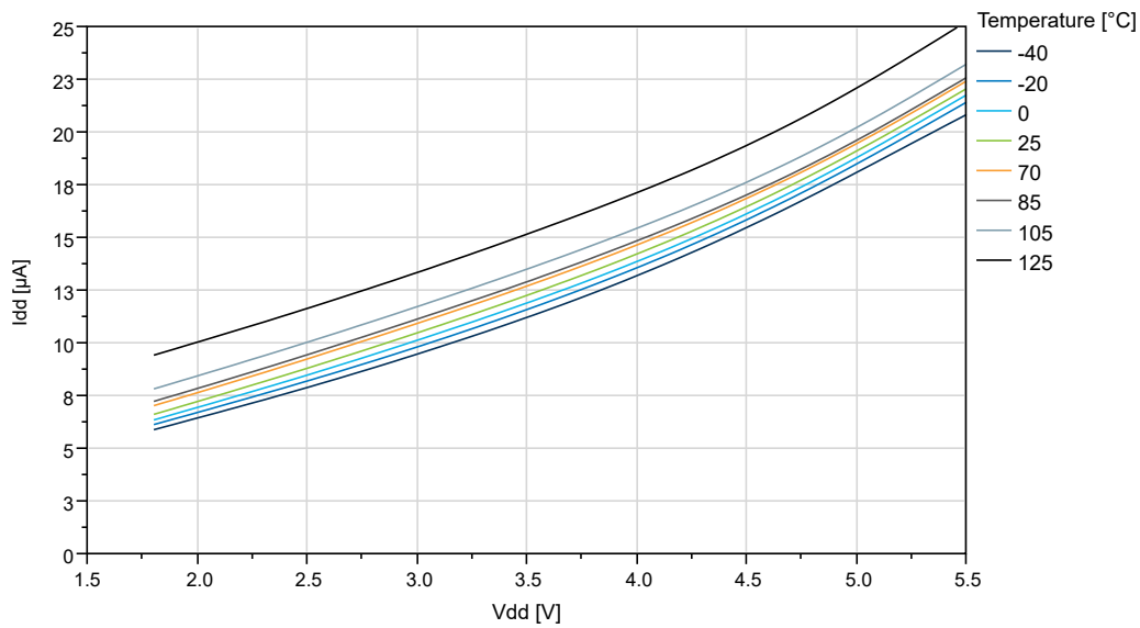
Figure 35-20. ATtiny816: Active Supply Current vs. V_{DD} ( f=32\text{KHz OSCULP32K} )
