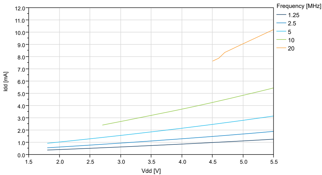
Figure 35-4. ATtiny416: Active Supply Current vs. V DD (f=[1.25, 20]MHz OSC20M) at T=25 ^{\circ}\text{C}
